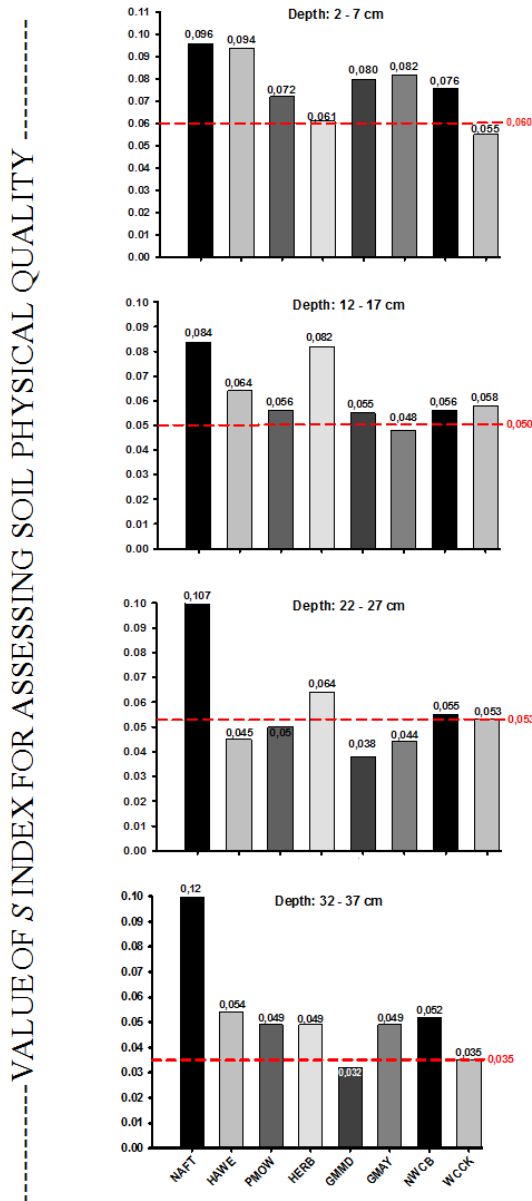
Figure 3. Soil physical quality “S index” for a Dystroferic Red Latosol in 2–7 cm, 12–17 cm, 22–27 cm and 32–37 cm layers, under natural forest and coffee plantation. NATF: native forest; HAWE: hand weeding; HERB: pre plus post-emergence herbicides; PMOW: portable mechanical mower; GMMD: dwarf mucuna ( Mucuna deeringiana ); GMAY: peanut horse ( Arachis hypogea ); NWCB: no-weed control between coffee rows; WCCK: weed check. The dotted horizontal line represents the critical value for S index in each soil layer.
